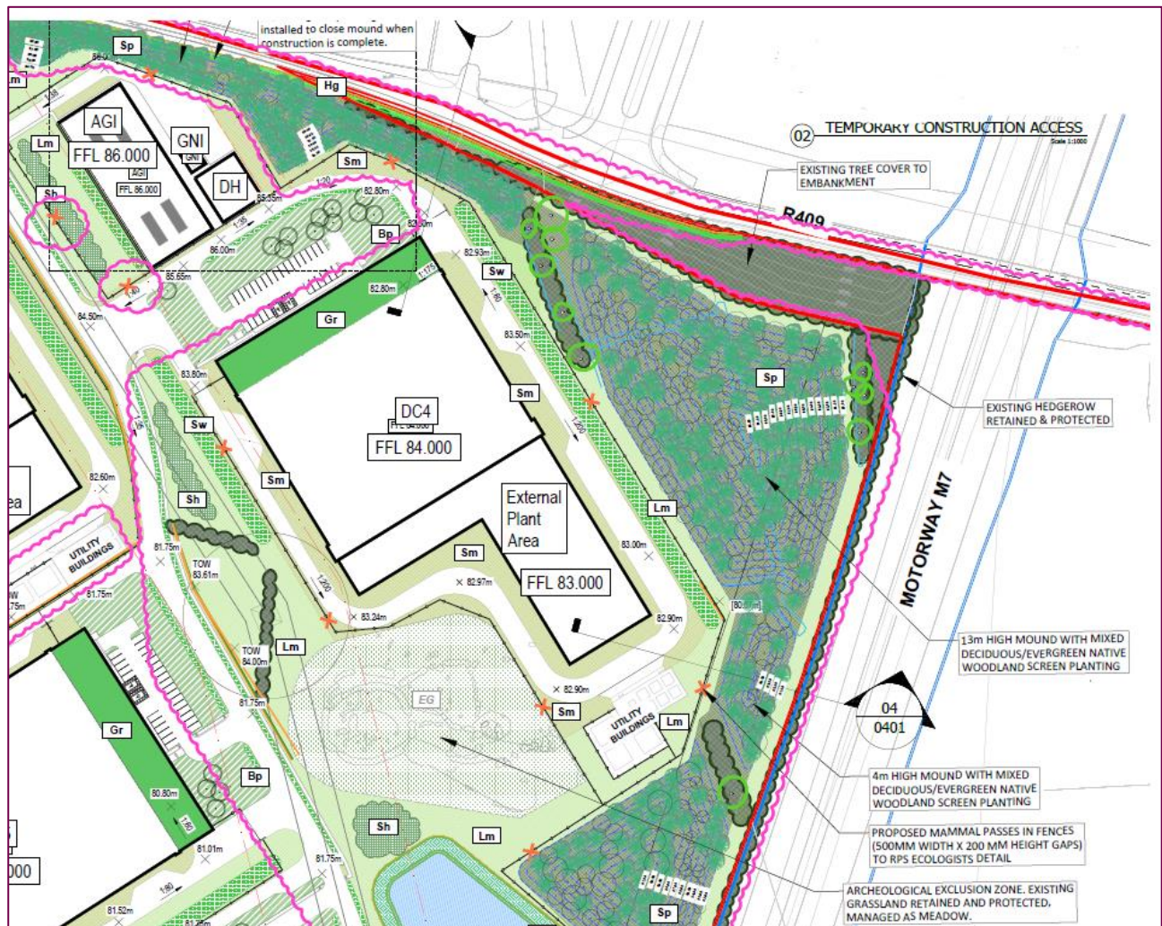
Figure 4.9: Landscape Proposals Relative to Amended Design of Data Centre 4 (extract of now submitted drawing BSM-ZZ-ZZ-DR-L-0301)
